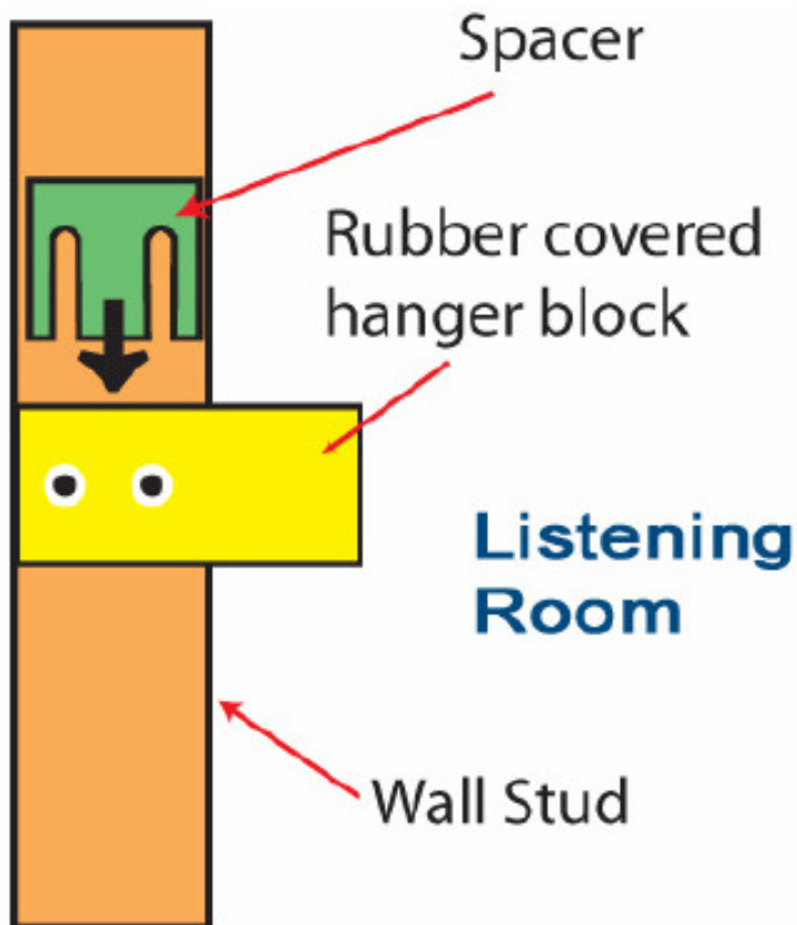
Side View Right Block Mounting
